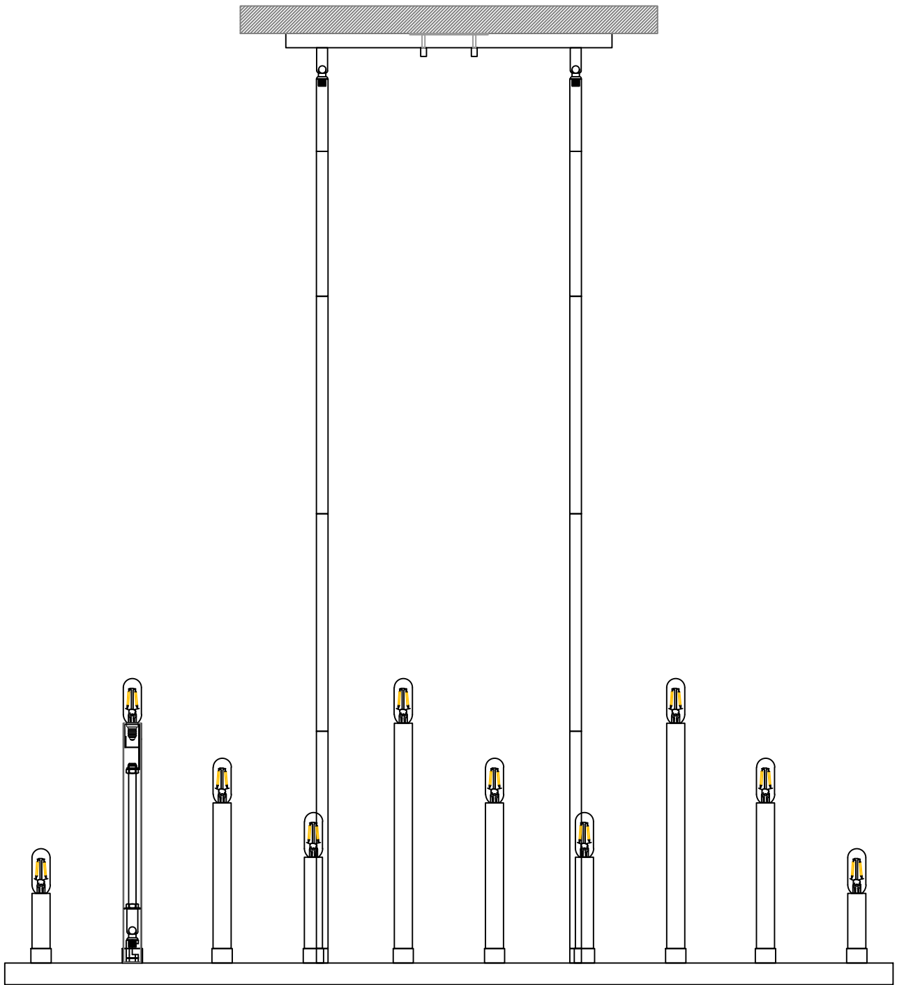
Front View
